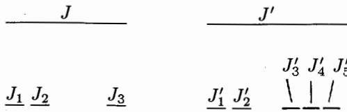
FIGURE 2. Splitting; q = 3, i = 3 .
